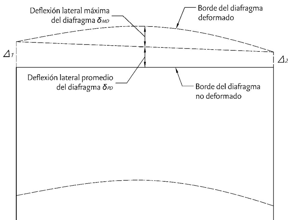
Figura 9. Diafragma flexible.
